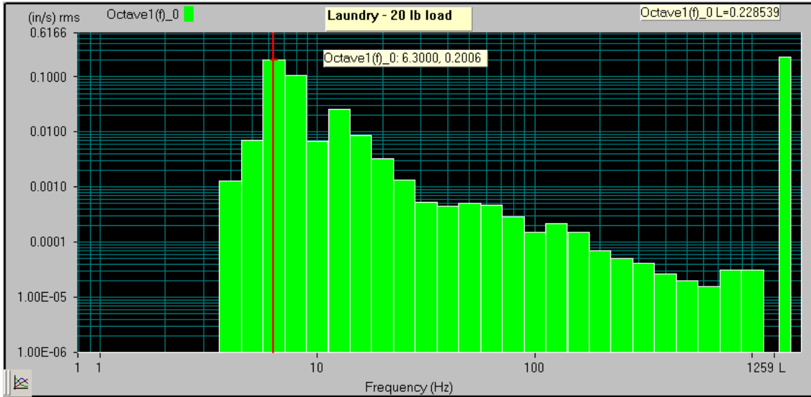
Figure 6: Vertical vibration with 20 lb. unbalanced load while accelerating to extraction RPM - 0.201 in/sec at 6.3 Hz.
