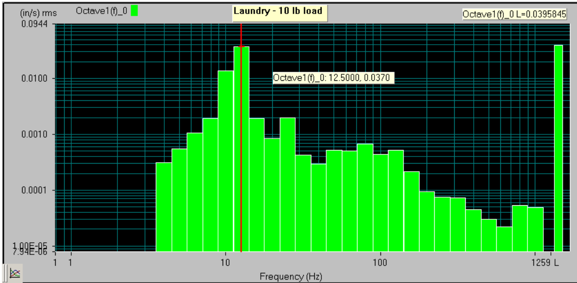
Figure 5: Vertical vibration with 10 lb. unbalanced load during steady extraction RPM - 0.037 in/sec at 12.5 Hz, slightly above criteria.
