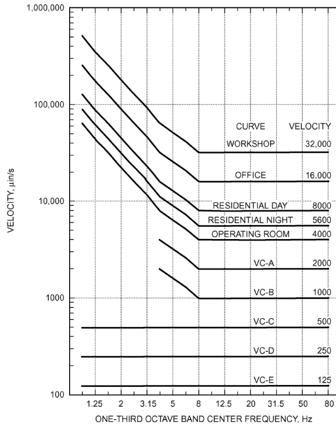
Figure 1: ASHRAE suggested vibration criteria for occupied buildings 2 .
