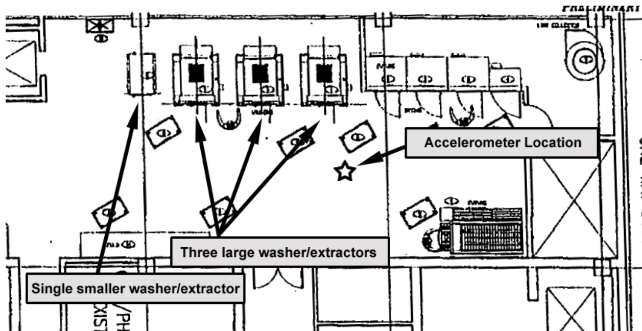
Figure 3: Floor plan of laundry services space.
