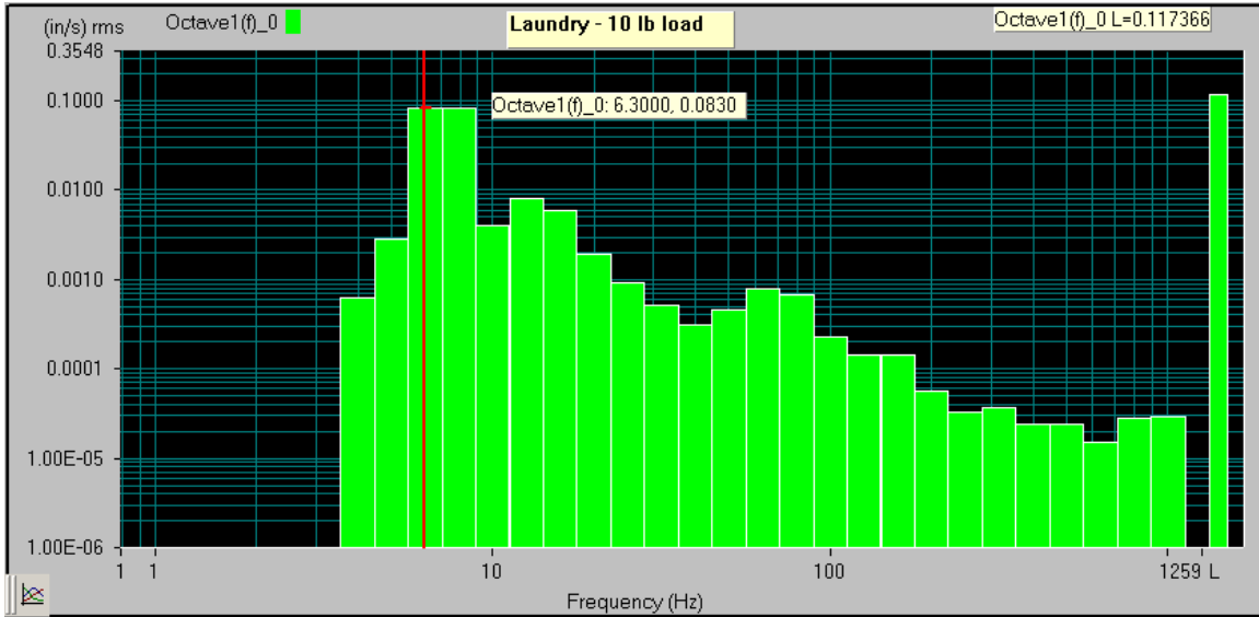
Figure 4: Vertical vibration with 10 lb. unbalanced load while accelerating to extraction RPM - 0.083 in/sec at 6.3 Hz and 8Hz, almost 3 times criteria.
