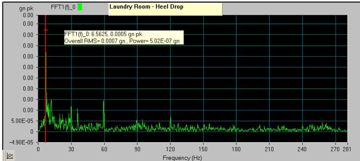
Figure 7: Heel drop test – natural frequency ( F_n ) of laundry floor slab = 6.56 Hz.
