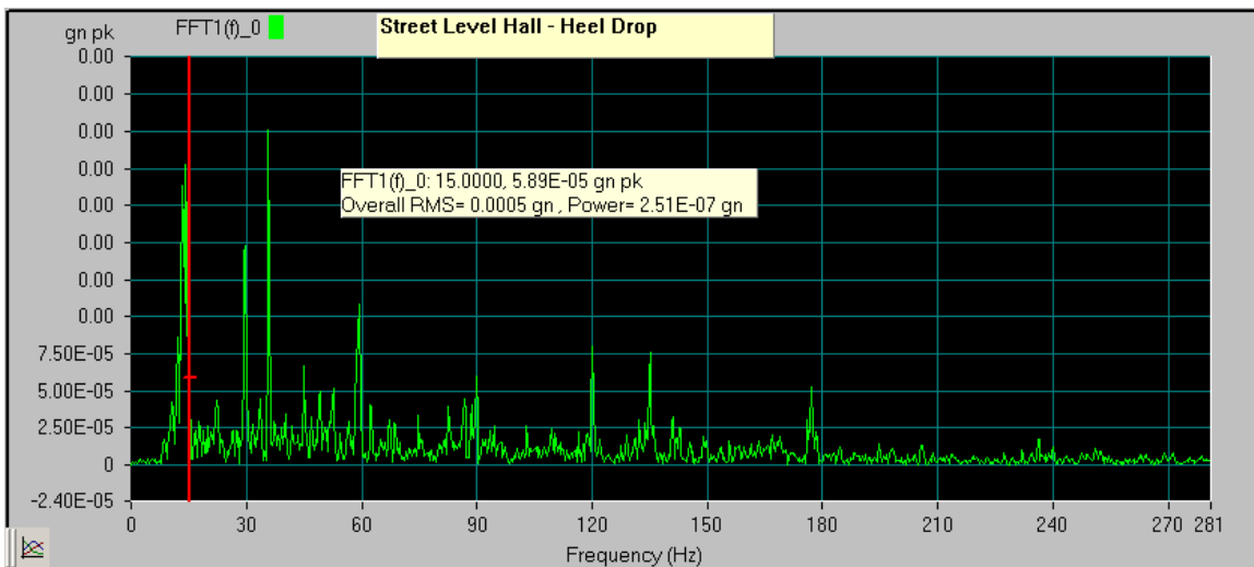
Figure 8: Heel drop test – natural frequency (Fn) of First Floor slab = 14 Hz.
